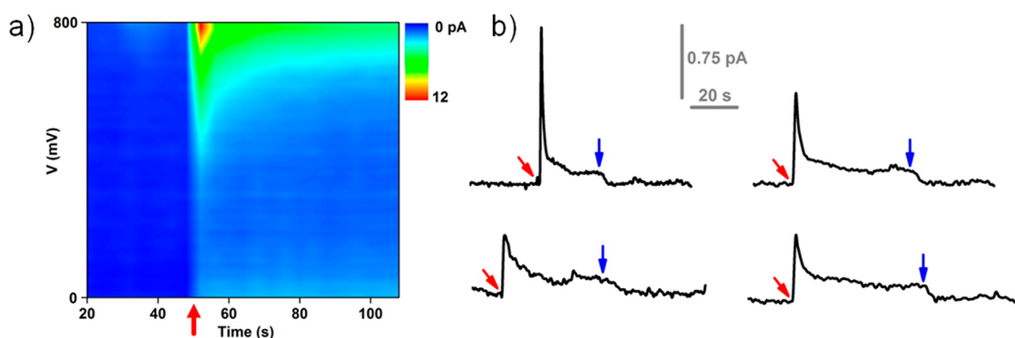
Figure 5. Intracellular measurements in individual neurons in a brain slice. (a) Background subtracted voltammograms before and after penetration of a neuron with the nano-electrode. Voltage is applied vs Ag/AgCl. (b) Representative current traces of a nano-electrode polarized at +850 vs Ag/AgCl inside and outside a neuron. Red and blue arrows indicated, respectively, the moment of penetration and retraction. The four traces were obtained from four different cells using the same nano-electrode.
